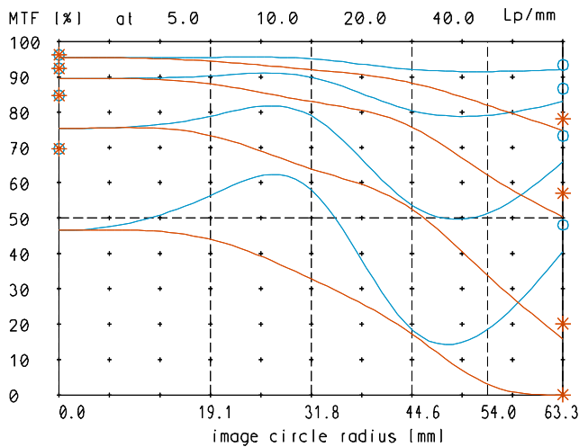
MTF at ratio infin f/ 11
