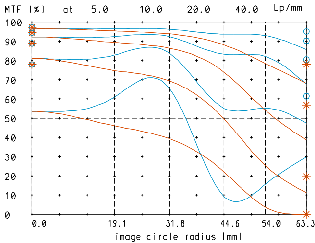
MTF at ratio infin f/ 8
