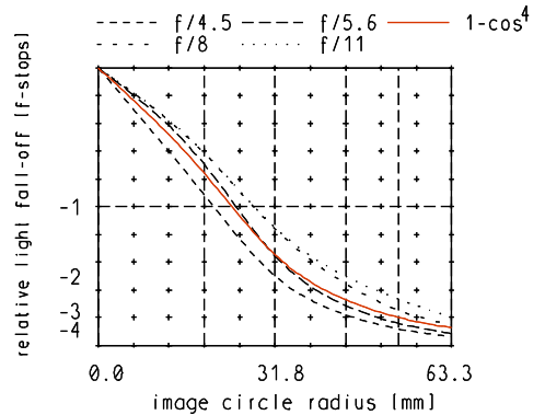
relative light fall-off at ratio infin
