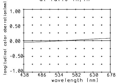
Longitudinal color aberration at ratio infin
