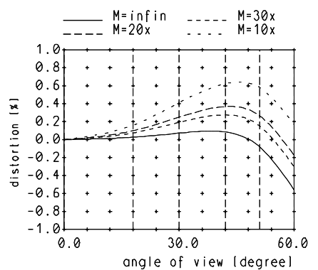
Distortion at ratio infin to 10x
